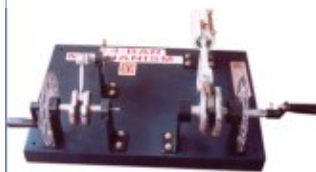
BSPIL-MOD-THR CRANK ROCKER MECHANISM
